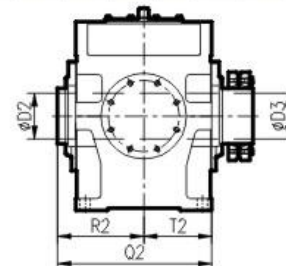
空心出力軸帶鎖緊盤型 Hollow Output Shaft (Shrink Disk Type)
