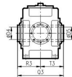
空心出力軸帶鍵 Hollow Output Shaft(Key Type)
