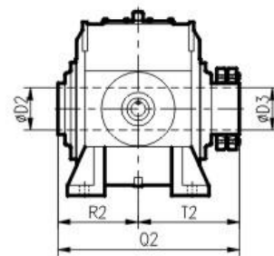
空心出力軸帶緊縮盤 Hollow Output Shaft (Shrink Disk Type)
