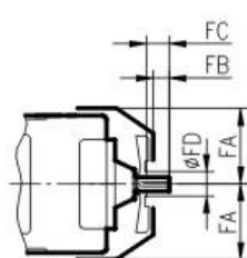
入力軸帶風扇 Input Shaft With fan
