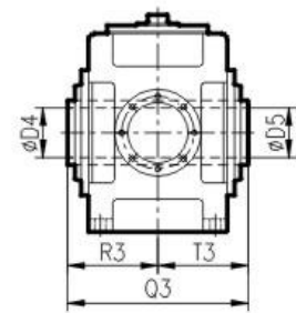
空心出力軸帶鍵 Hollow Output Shaft(Key Type)
