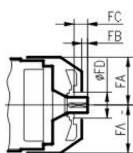
入力軸帶風扇 Input Shaft With fan
