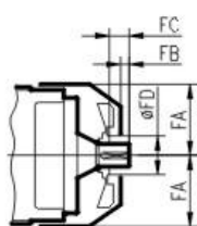
入力軸帶風扇 Input Shaft With fan
